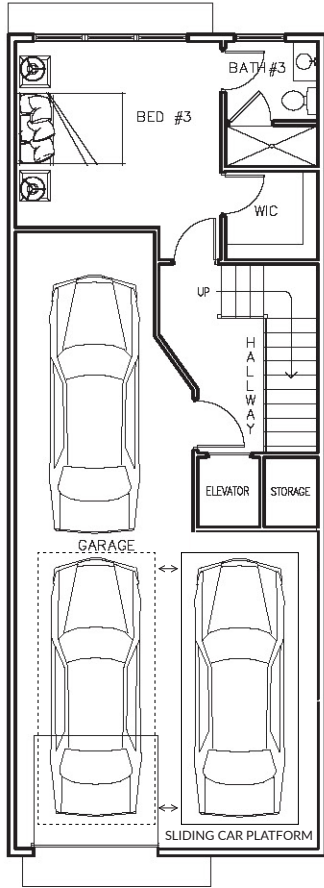
1st Floor
